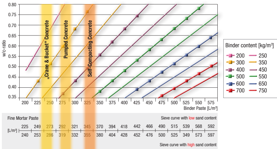
Fig. 4.2.1: Relation between concrete compressive strengths of a specific cement, expressed in w/c-ratio, and the fine mortar quantity (L/m³) for a required cement content (kg/m³)
