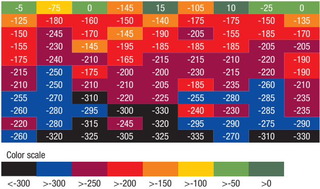
Fig. 8.2.4: Potential measurement on a retaining wall along a road with heavy traffic with high use of de-icing salt, after less than 10 years of exposure. The darker the coloration, the higher the potential for corrosion.
