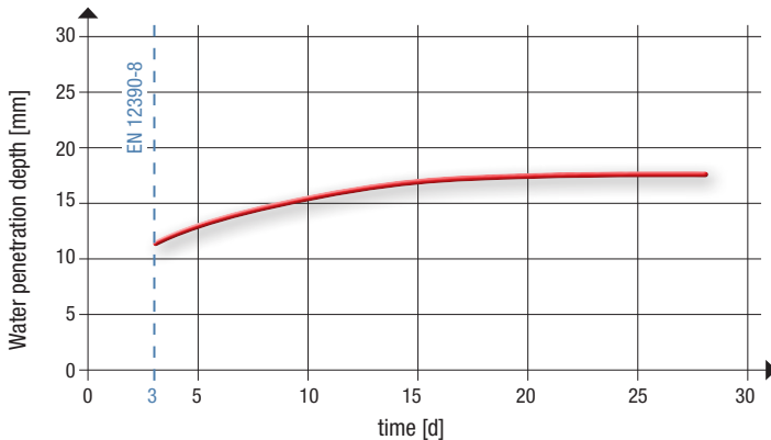
Fig. 7.8.5: Water penetration depth under 5 bar pressure over time
