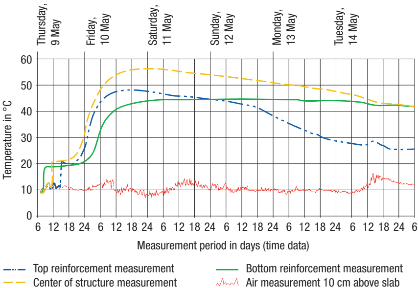
Fig. 6.5.1: Measurement of hydration heat in a 160 cm thick ground slab placed in three levels
