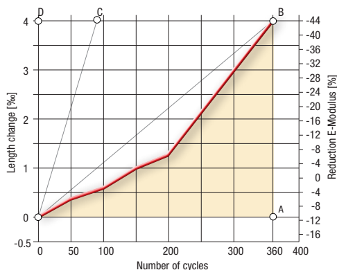
Fig. 8.3.2: In test BE II according to D-R 400, the test prisms are subject to alternating loads between +20°C and -20°C, the change in length is measured and judged between three ranges of durability (low / middle / high). Calculation according to ASTM C666.
