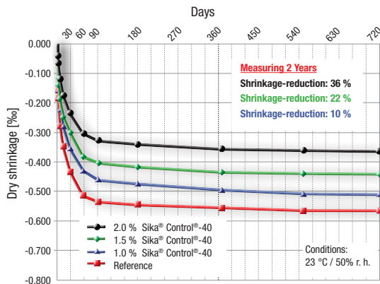
Fig. 8.10.1: Shrinkage behaviour of concrete containing shrinkage-reducing admixtures, measured up to 2 years to complete abatement of shrinkage due to drying.
