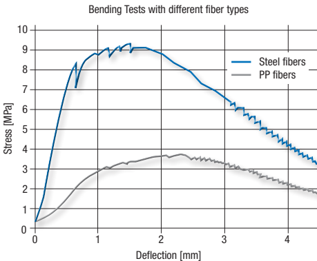
Fig. 8.11.2: The stress-deflection diagram of a bending test shows the influence of different fiber types on the material properties of the concrete, like improved tensile strength and a well controlled post cracking behavior.
