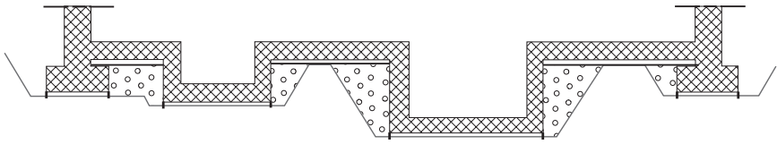
Figure 9.1: Traditional design of reinforced concrete base slab, not suitable for 'White Box' concept
