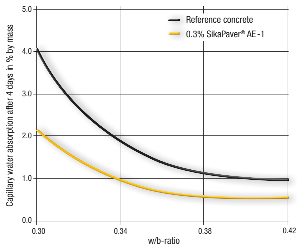
Fig. 6.12.3: Influence of SikaPaver® AE-1 on capillary absorption
