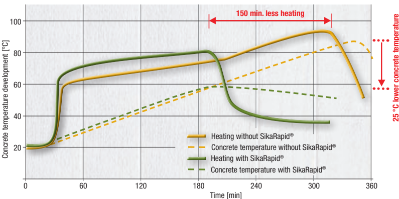
Fig. 6.10.1: Heating development and development of concrete temperature
