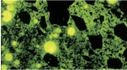
Fig. 7.8.4: Porosity of concrete at different w/c-ratios
