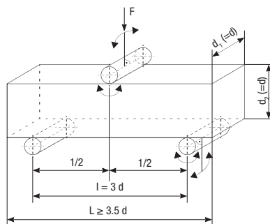
Fig. 7.4.2: Central load transfer
