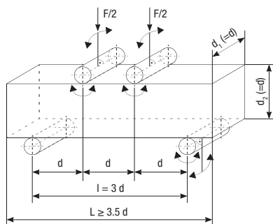
Fig. 7.4.1: Two-point load transfer
