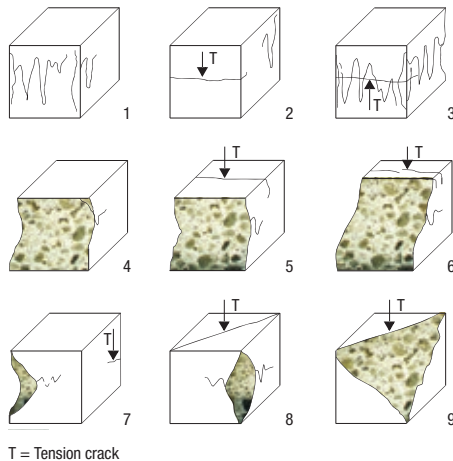
Fig. 7.3.3: Unusual break patterns on cubes (illustrations from the standard)
