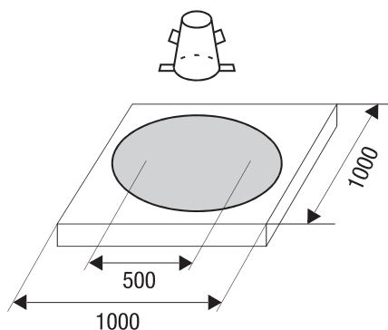
Fig. 5.2.7: Slump-flow test
