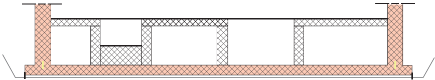
Figure 9.2: Appropriate design for 'White Box': simple tank shape, homogenous thickness, no offsets. The red part will be designed in high quality concrete (watertight concrete)
