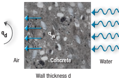
Fig. 8.1.3: Immersion and permanent water contact. The water permeability limit for watertightness is defined as 10 g/(m 2 x hours) (according to SIA 262/1), where water permeability is smaller than vaporizable volume of water without pressure over a defined period.
